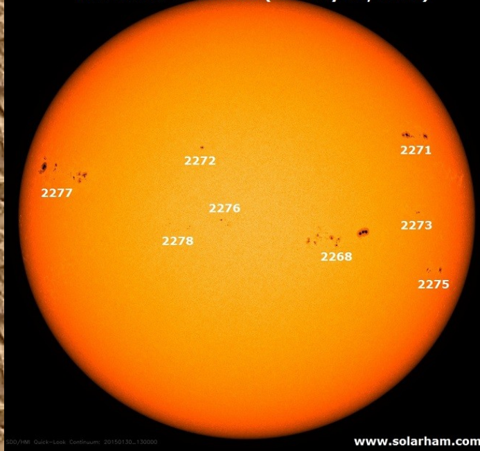
The Visible Solar Disk (January 30, 2015)
